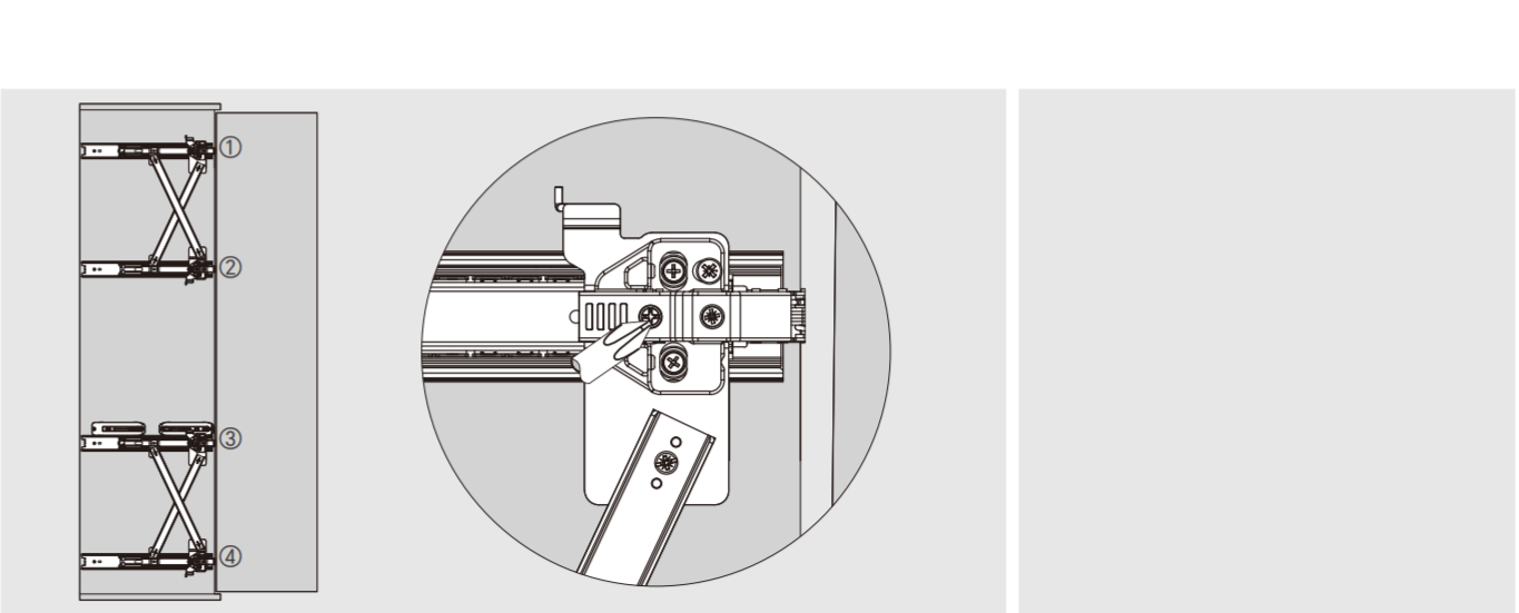
Adjust the screw No. ①③ to make the door move inside Adjust the screw No. ②④ to make the door move outside
