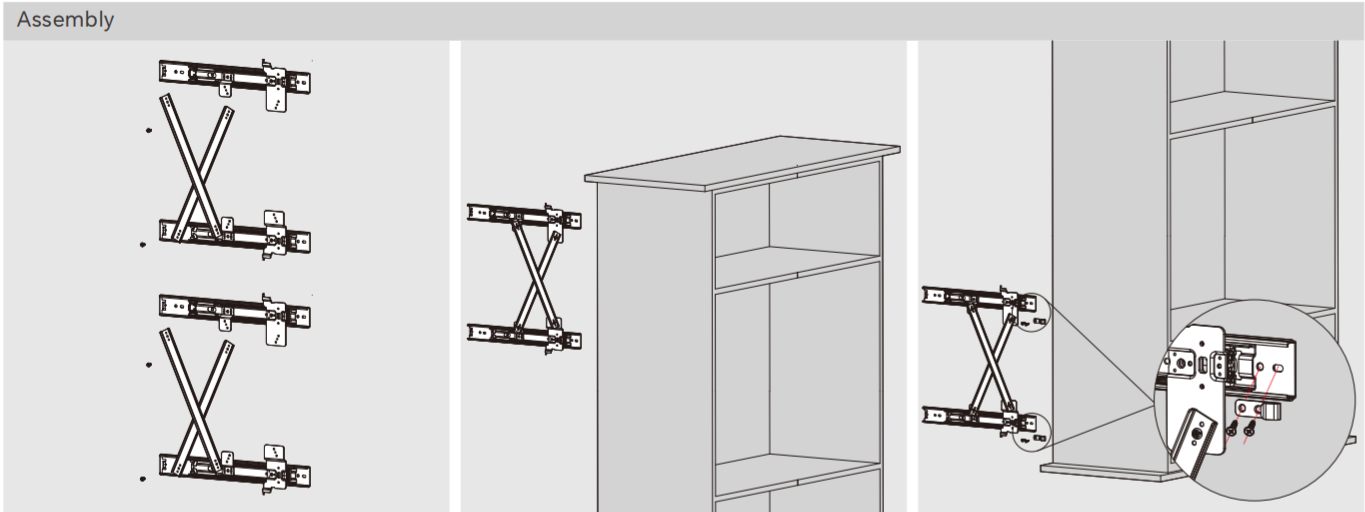
Install cross bars Install the slide on the inner side board Install stopper (please install the stopper at the bottom set of slides)
