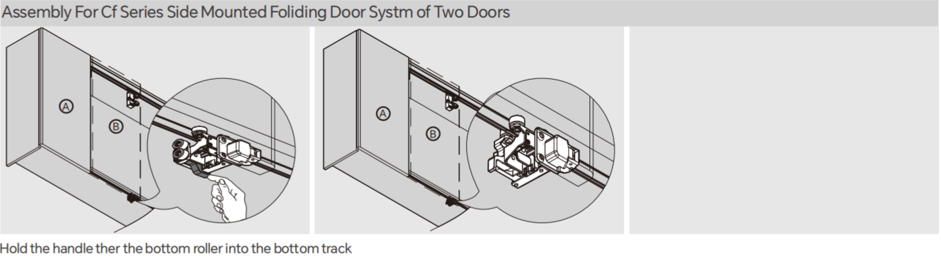
Hold the handle then the bottom roller into the bottom track
