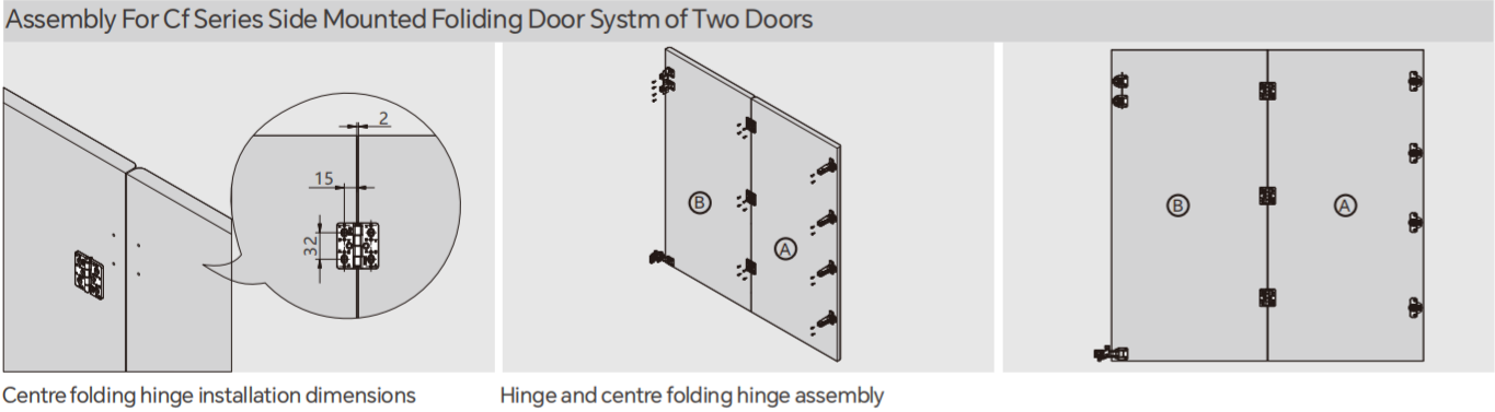
Centre folding hinge installation dimensions
